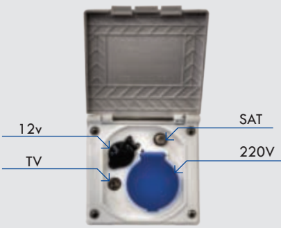
Multifunction external socket for TV, 12V, 220V and Satellite.
